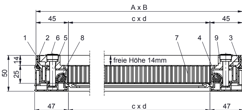
Typ CLA-SL slim composite light Alu
